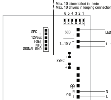
1...10 V diagram - Collegamento 1...10 V
